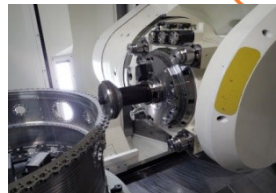
Under Machining
